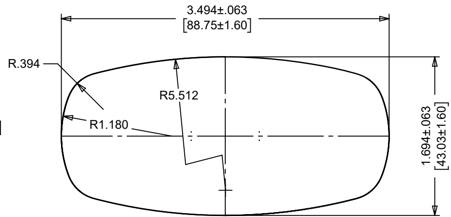
SECTION VIEW AT .591 UP FROM BOTTOM
