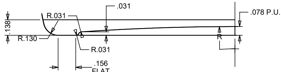
BOTTOM CAVITY DETAIL SCALE 2 : 1
