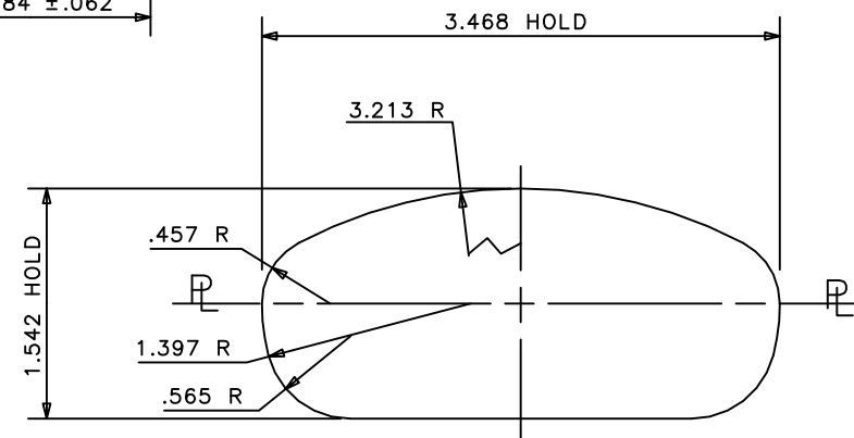
SECTION AT .125 UP
