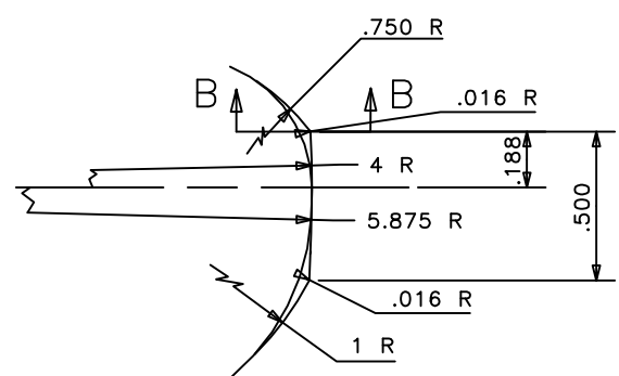
BUMPER PAD DETAIL SCALE: 2 TO 1
