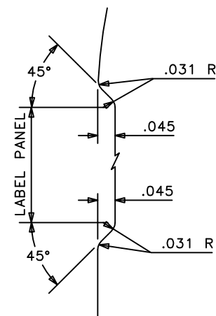
LABEL INDENT DETAIL SCALE: 4 TO 1
