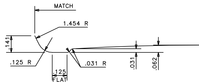
BOTTOM CAVITY DETAIL SCALE: 3 TO 1
