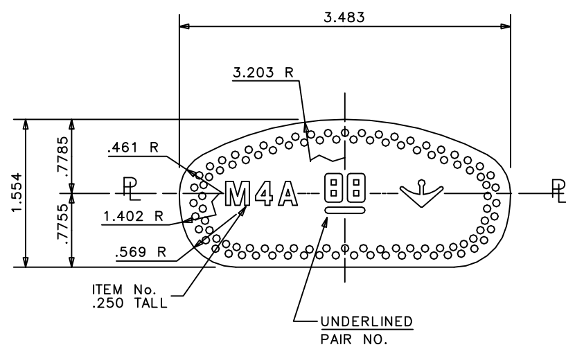
SECTION AT .141 UP MOULD & BOTTOM MATCH
